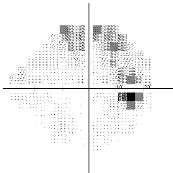
MD Progression(DB)
