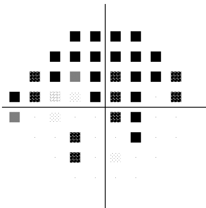
Total Deviation
