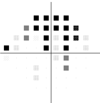
Pattern Deviation
